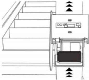
C. The rear roller and the handrail's rotational force generates power
